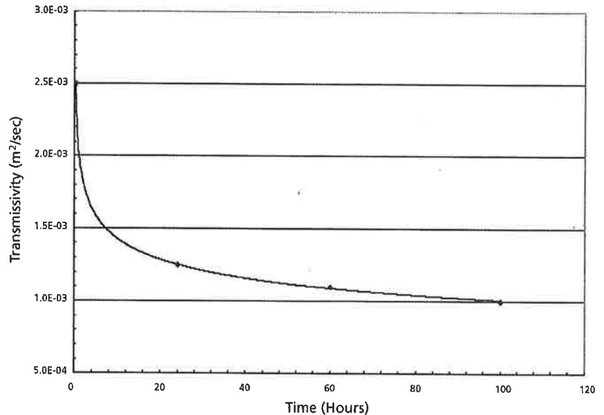
Figure 2. Typical transmissivity behavior of synthetic drainage products with time. From Narejo and Richardson (2003).
