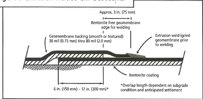
Figure 3: Extrusion-welded GM-GCL seams.
