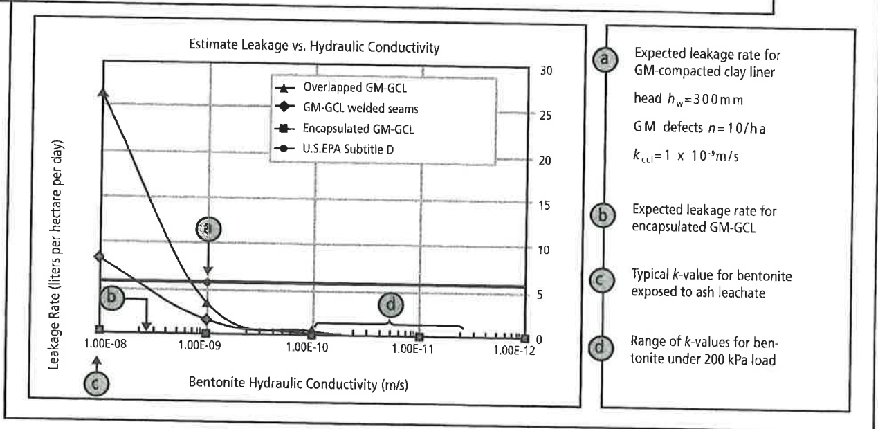
Figure 8: Comparison of hydraulic performance of example composite bottom liner systems with (a) GM-GCL alternative liners and (b) U.S. EPA Subtitle D composite bottom liners.
