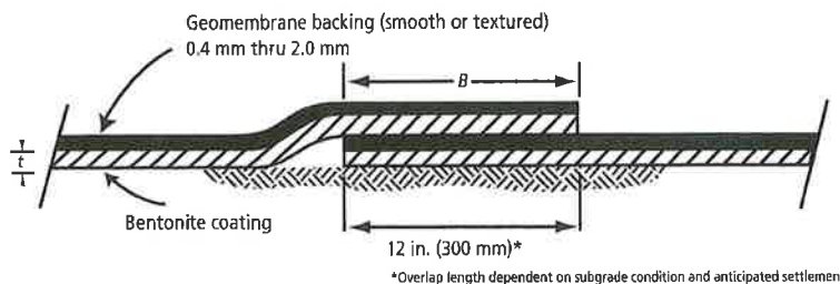
Figure 2: Overlapped GM-GCL with shingle seams.
