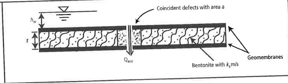
Figure 7: Drawing illustrating the factors taken into account by the equation, derived from Darcy's law, for estimating seepage at overlapped (unwelded) GM-GCL seams.
